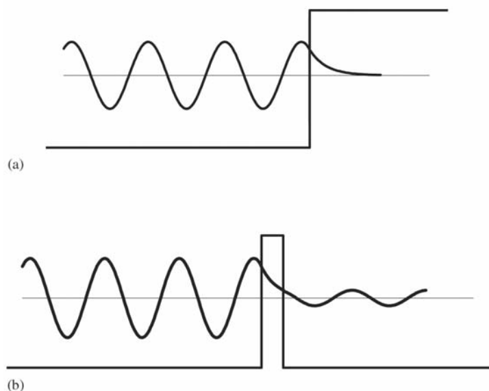
Figure 2.6 The strong straight lines in (a) represent a potential step. The wave function for a particle approaching the step is also shown; it penetrates the step, giving a probability of finding the particle in a region that is forbidden classically. The corresponding case for a narrow barrier is shown in (b) the wave function penetrates the barrier so that there is a probability of the particle emerging on the right-hand side, where it could never be classically. This is known as ‘quantum mechanical tunnelling’.
