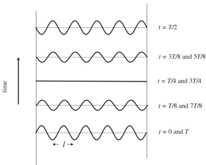
Figure 2.3 Standing waves occur when a wave is confined to a region in space. The wave moves up and down in time but not in space.
