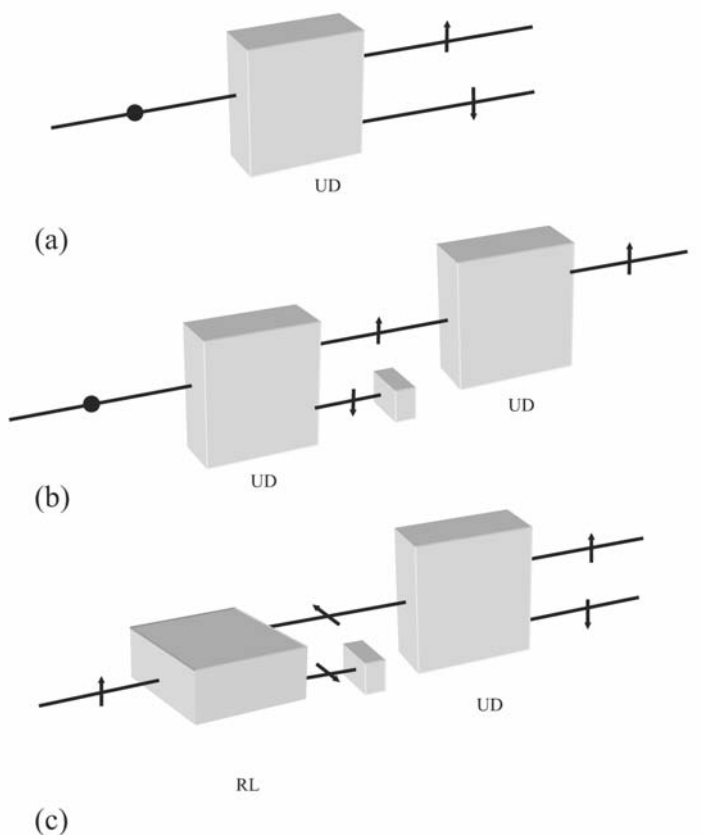
Figure 7.1 The boxes represent Stern–Gerlach magnets. A particle passing through them emerges in one channel or the other depending on the direction of its spin. (a) represents a measurement of the up/down (UD) spin. Once the spin direction is known, subsequent measurements in the same direction give the same answer (b). In (c) particles previously found to have their spins pointing up pass through a left/right (LR) polarizer and emerge from either channel at random. The act of measuring the LR polarization has also destroyed our previous knowledge of its UD state, so the photons again emerge at random when this spin is measured.
