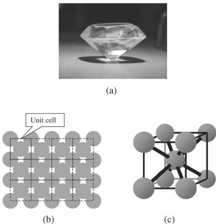
Figure 4.4 Crystals and their atomic structures. A single crystal of diamond is shown in (a). In (b) we see how disks can be arranged to form a square pattern that repeats itself across the plane of the page. Similarly, in three dimensions spheres can pack together to form a cubic unit cell and this is illustrated in (c) (where, for clarity, touching spheres are replaced by smaller spheres connected by rods). An example of this structure is that of a crystal of copper.
