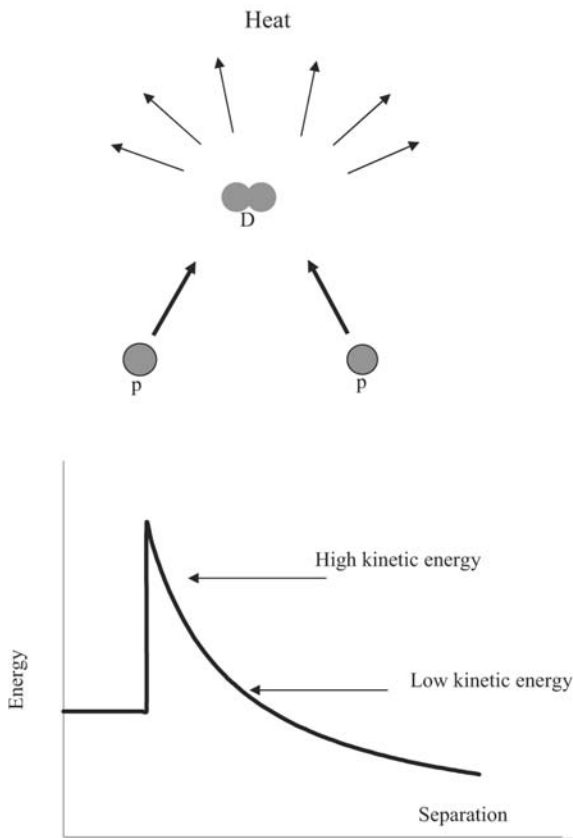
Figure 3.2 When two protons fuse together to form a deuterium nucleus (De), energy is released and a positron and neutrino (neither are shown above) are emitted. However, before this can occur, they must tunnel through the potential barrier created by the electrostatic repulsion. The probability of this happening is very low, unless the protons approach each other at high speed and therefore high kinetic energy, which makes the effective barrier lower and narrower. Note: the scale of this diagram is about two thousand times larger than that in Figure 3.1 and the energy released is about a million times greater.
