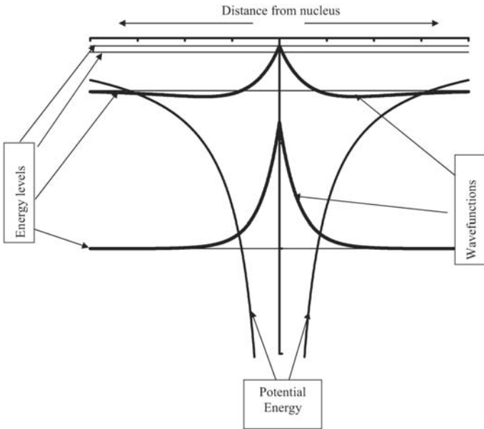
Figure 2.9 The hydrogen atom. The diagram shows the potential energy along with the four lowest energy levels and the wave functions corresponding to the lowest two of these; the wave functions have been drawn so that their zeros are at the corresponding energy levels. Note that the zero of energy corresponds to the top line in the diagram.
